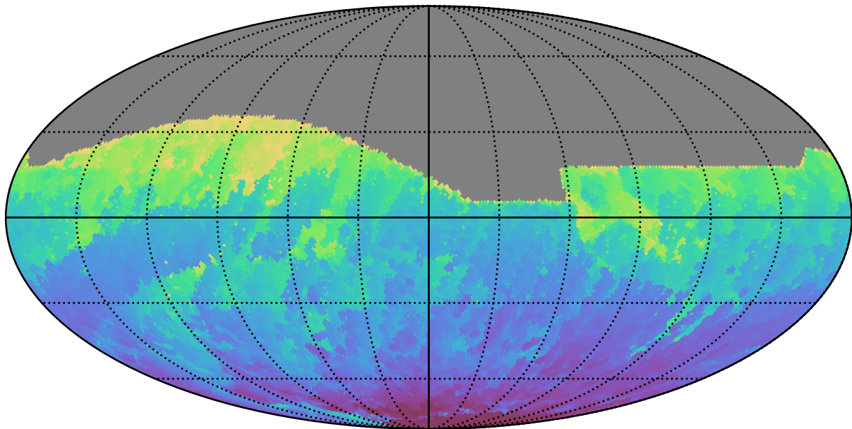
early_u_fpextra3.0_v3.4_10yrs All sky i band: Min HA
