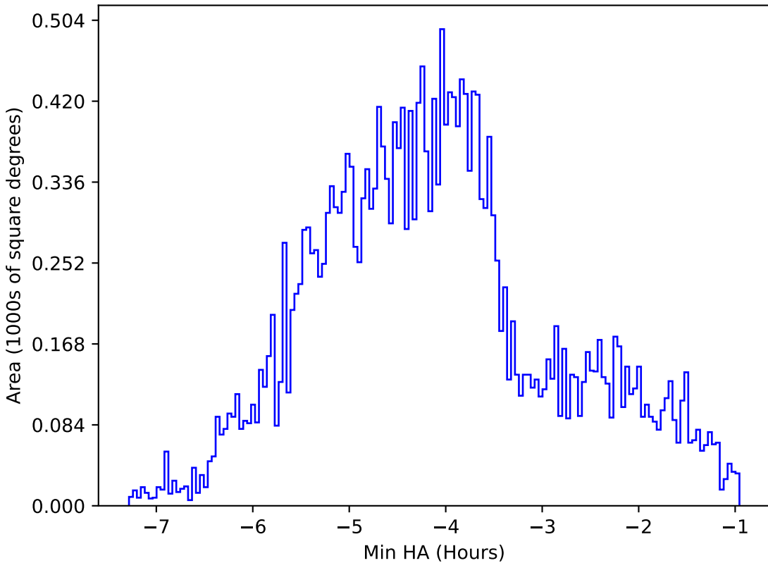
early_u_fpextra3.0_v3.4_10yrs All sky i band: Min HA
