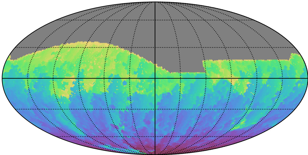
early_u_fpextra3.0_v3.4_10yrs All sky g band: Min HA
