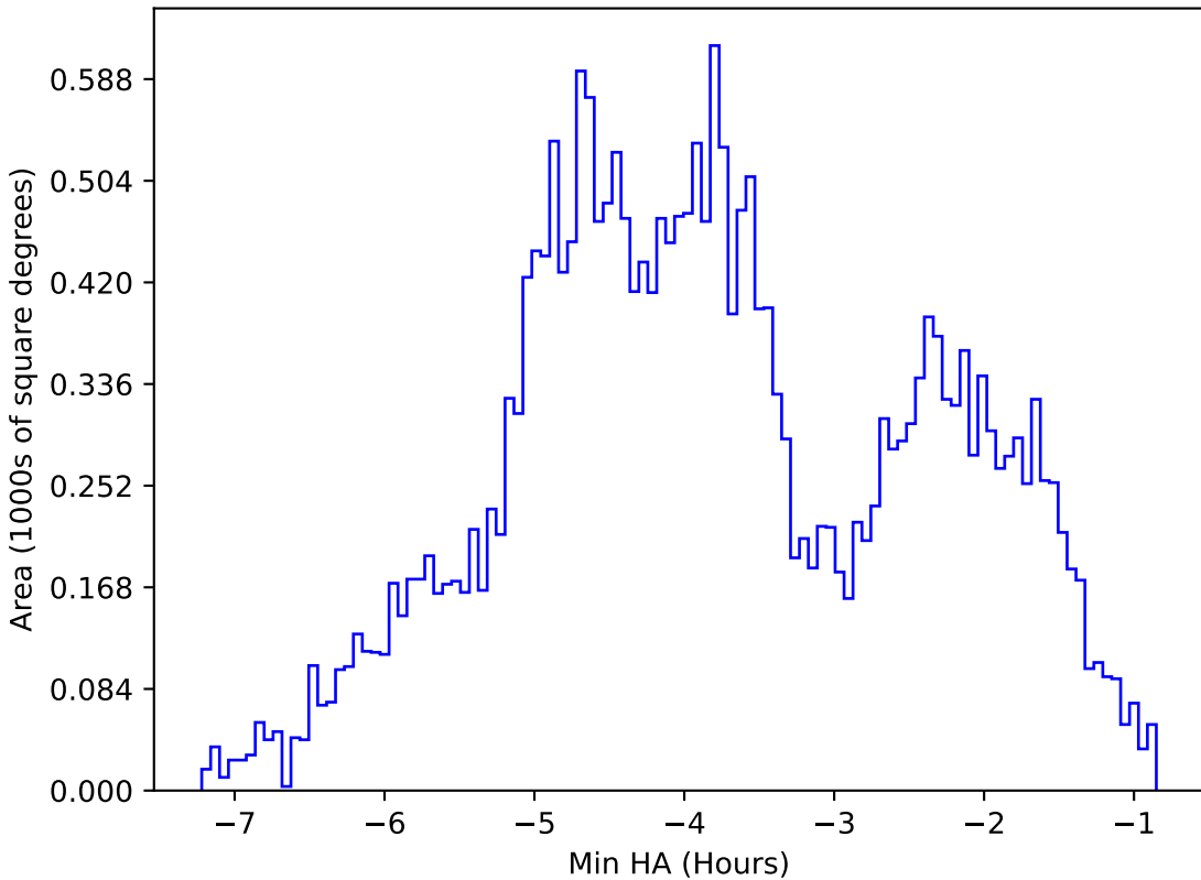
early_u_fpextra3.0_v3.4_10yrs All sky g band: Min HA
