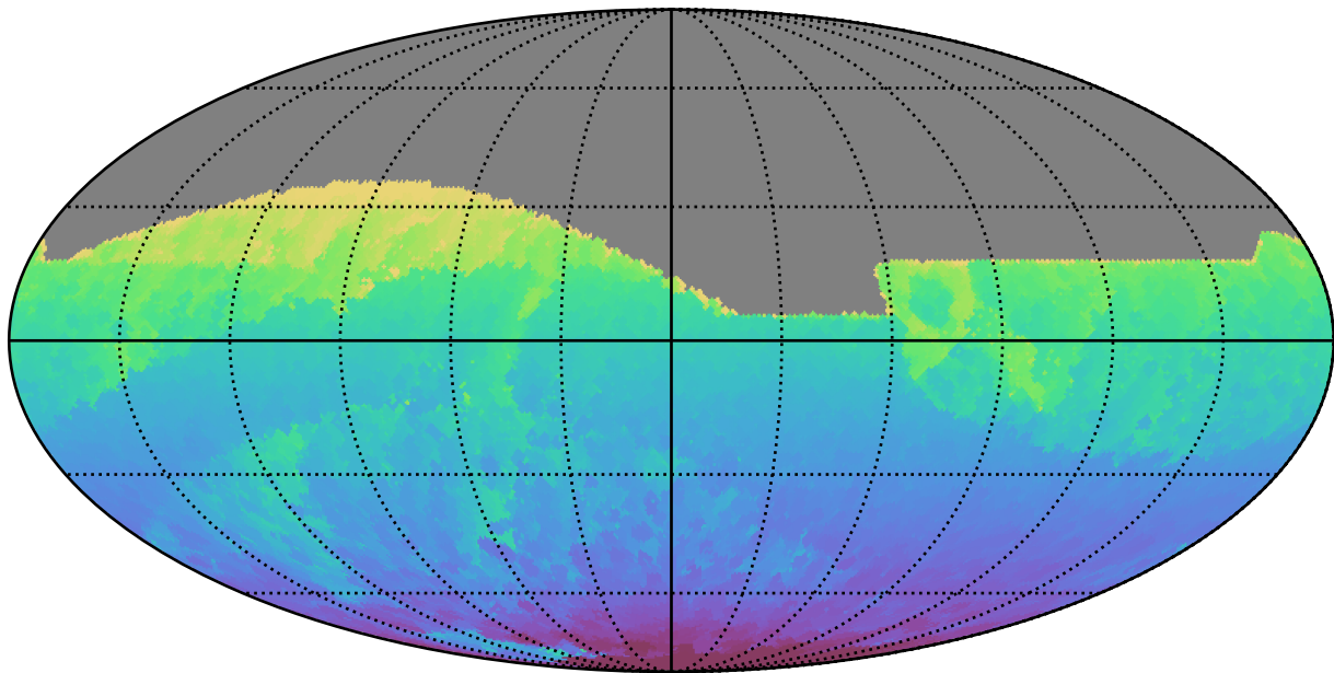
early_u_fpextra3.0_v3.4_10yrs All sky all bands: Min HA
