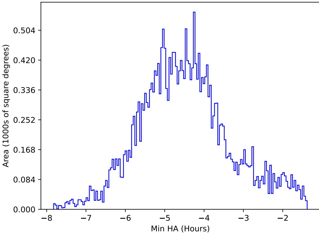
early_u_fpextra3.0_v3.4_10yrs All sky all bands: Min HA
