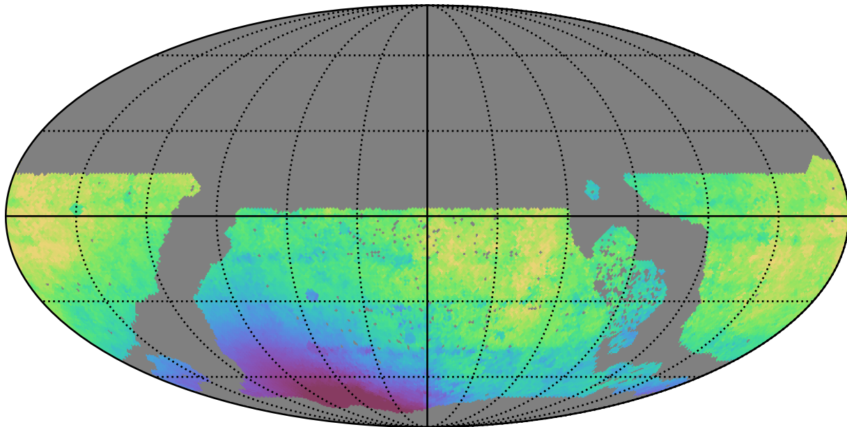
early_u_fpextra3.0_v3.4_10yrs WFD z band: Median solarElong
