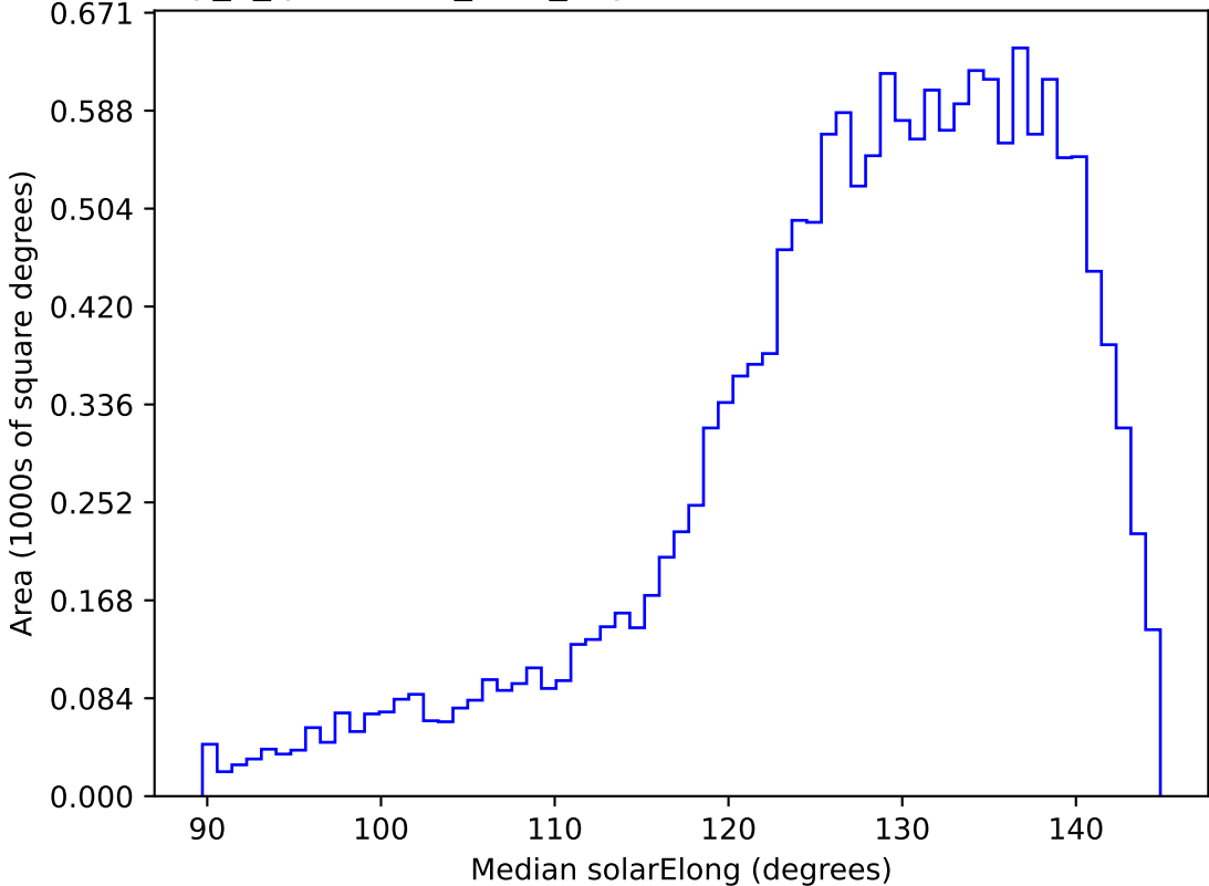
early_u_fpextra3.0_v3.4_10yrs WFD z band: Median solarElong
