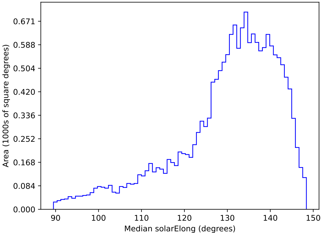
early_u_fpextra3.0_v3.4_10yrs WFD y band: Median solarElong
