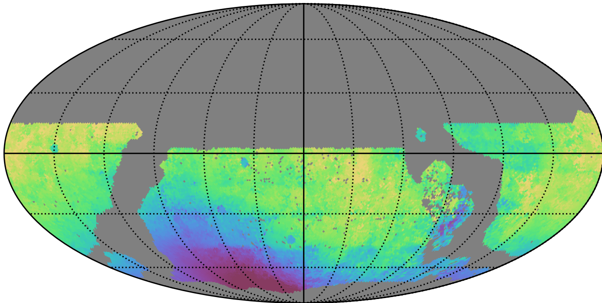
early_u_fpextra3.0_v3.4_10yrs WFD u band: Median solarElong
