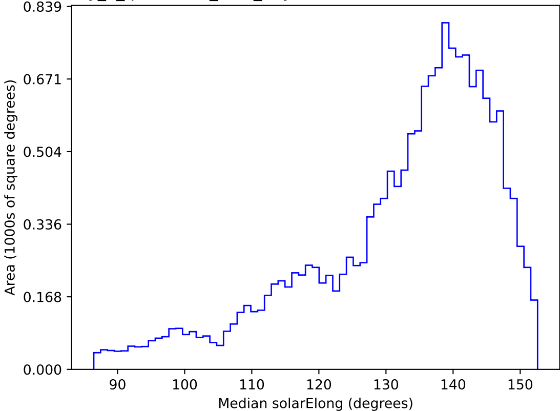
early_u_fpextra3.0_v3.4_10yrs WFD u band: Median solarElong
