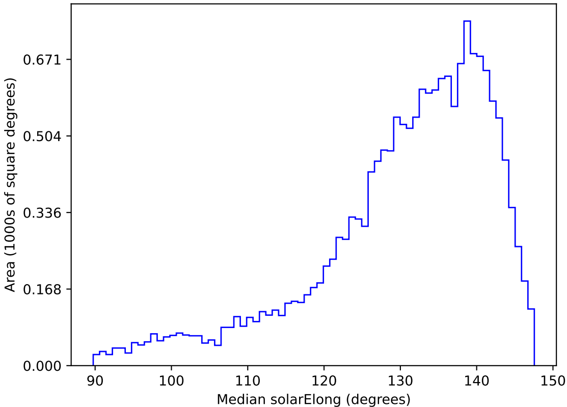
early_u_fpextra3.0_v3.4_10yrs WFD r band: Median solarElong
