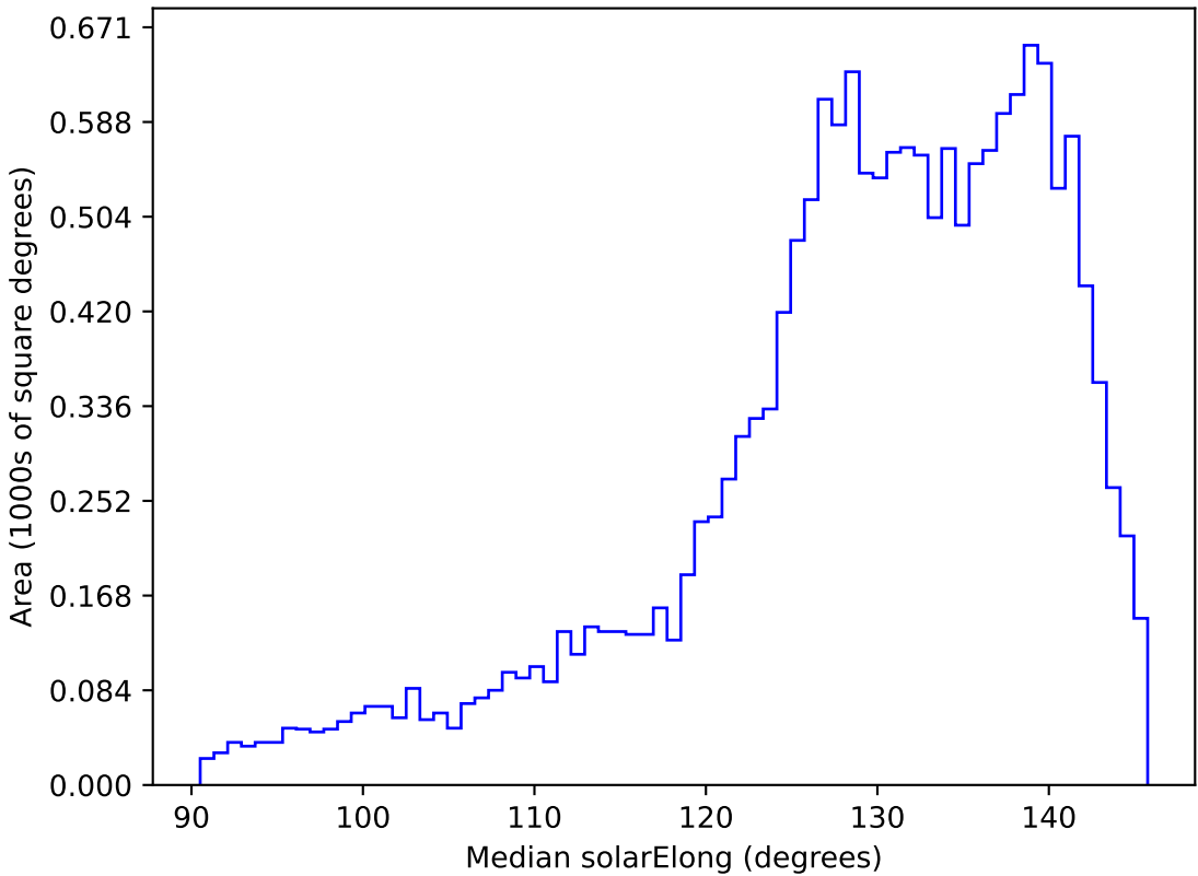
early_u_fpextra3.0_v3.4_10yrs WFD i band: Median solarElong
