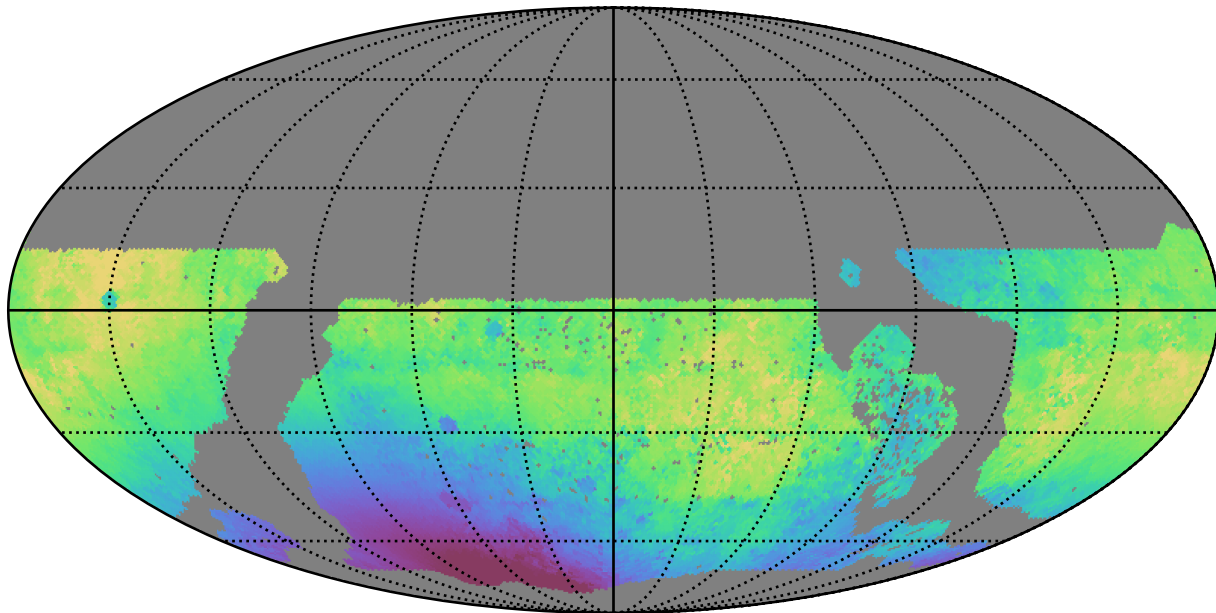
early_u_fpextra3.0_v3.4_10yrs WFD g band: Median solarElong
