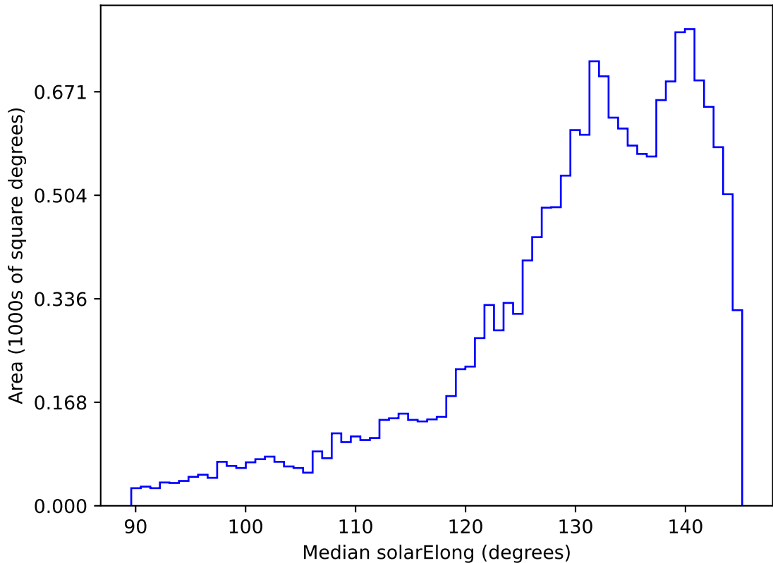
early_u_fpextra3.0_v3.4_10yrs WFD all bands: Median solarElong
