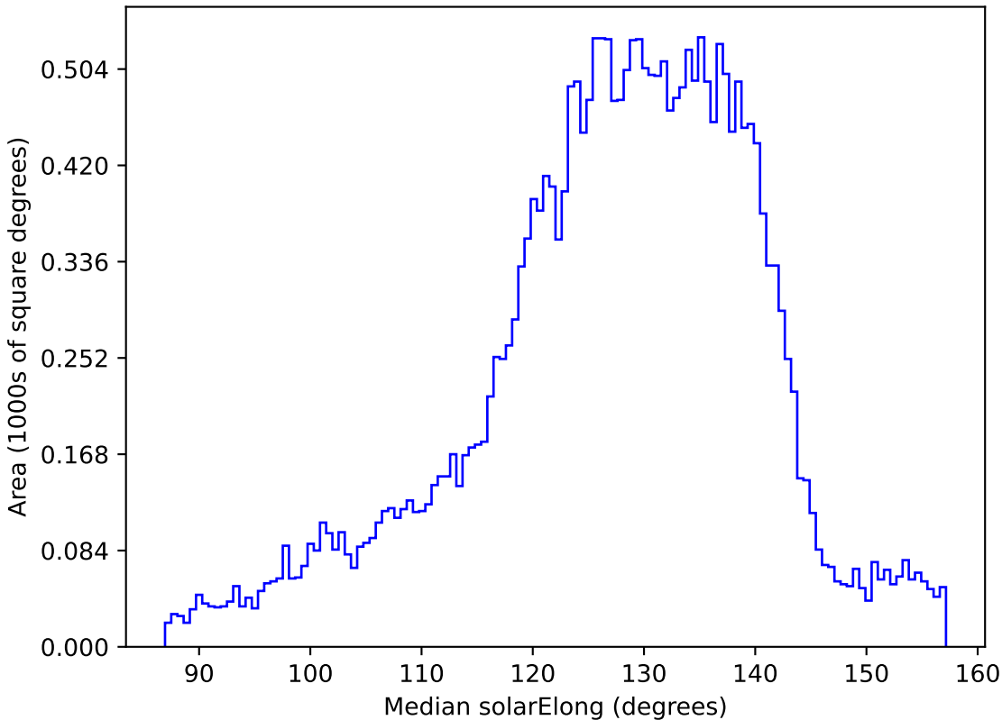
early_u_fpextra3.0_v3.4_10yrs All sky z band: Median solarElong
