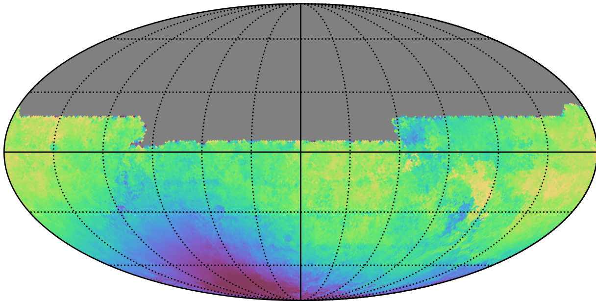
early_u_fpextra3.0_v3.4_10yrs All sky y band: Median solarElong
