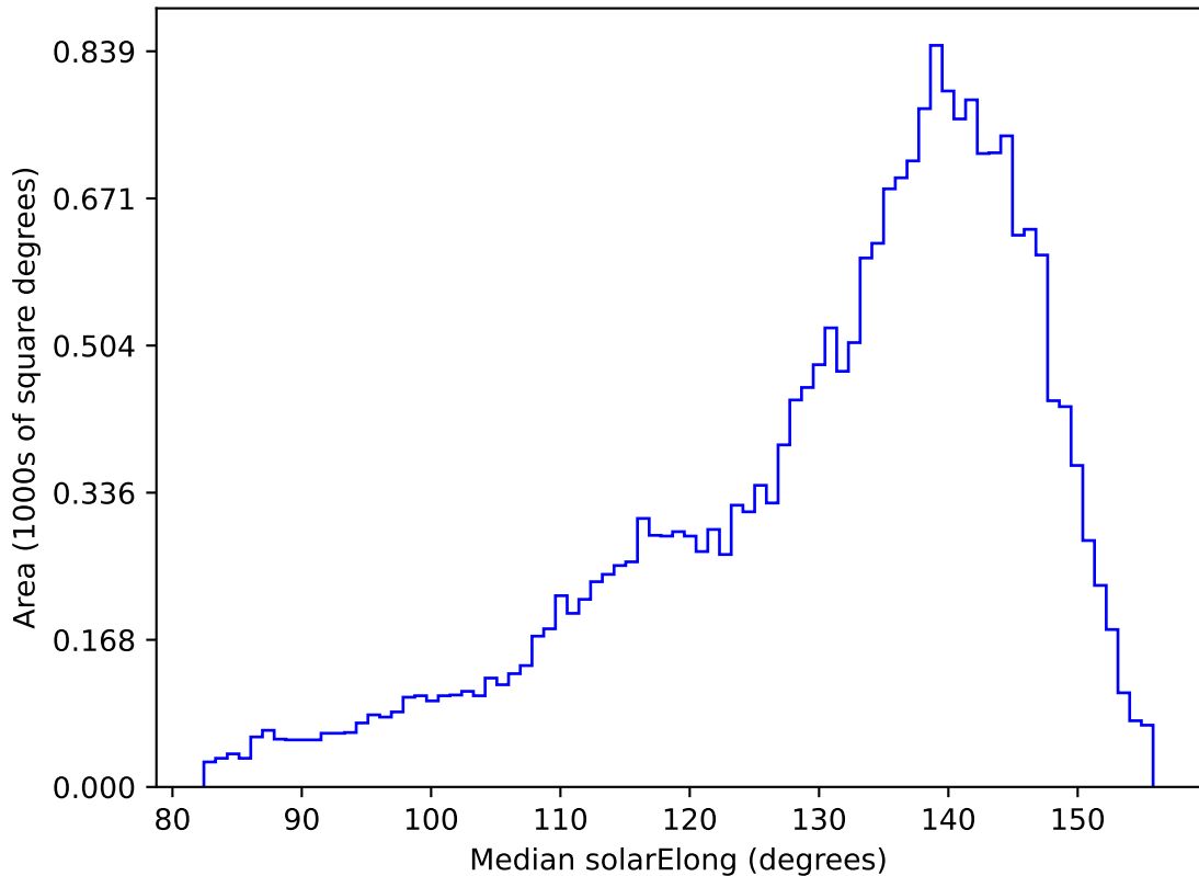
early_u_fpextra3.0_v3.4_10yrs All sky u band: Median solarElong
