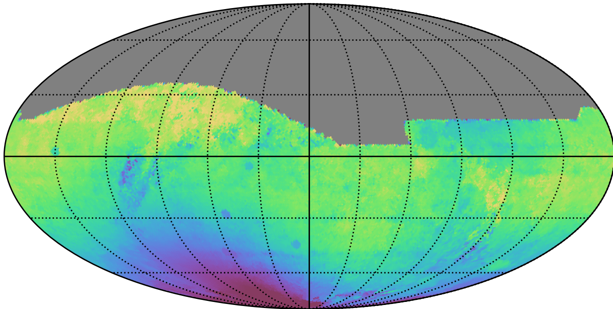
early_u_fpextra3.0_v3.4_10yrs All sky r band: Median solarElong
