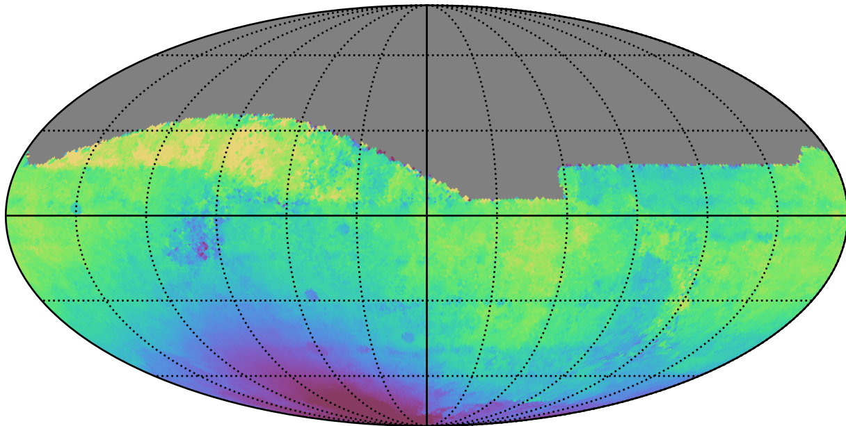
early_u_fpextra3.0_v3.4_10yrs All sky i band: Median solarElong
