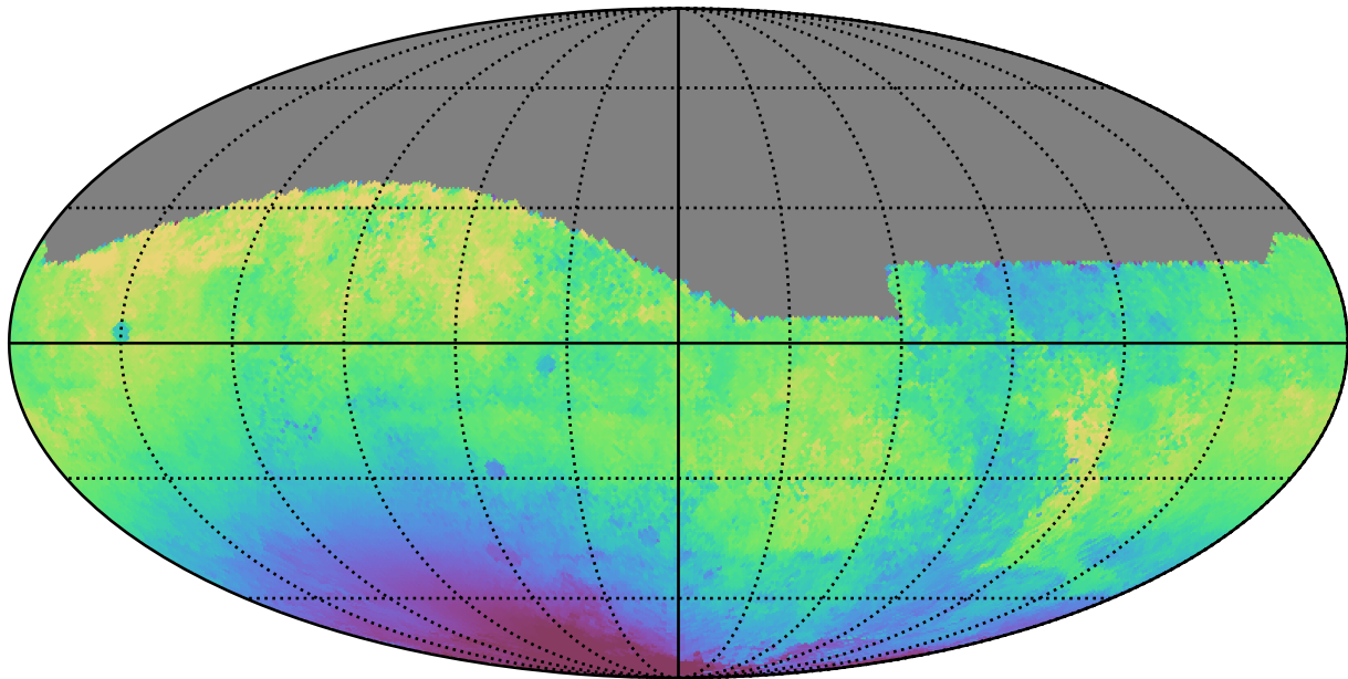
early_u_fpextra3.0_v3.4_10yrs All sky g band: Median solarElong
