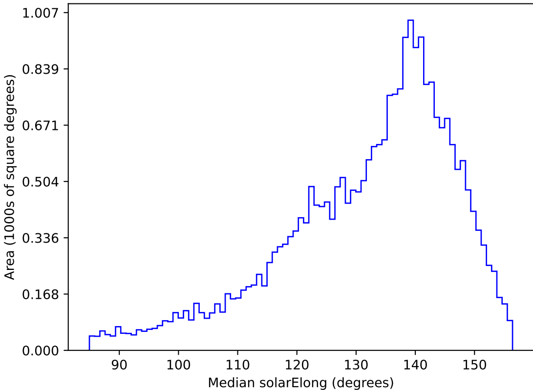
early_u_fpextra3.0_v3.4_10yrs All sky g band: Median solarElong
