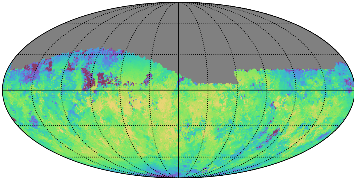
early_u_fpextra3.0_v3.4_10yrs Yr 1 z band: Median skyBrightness
