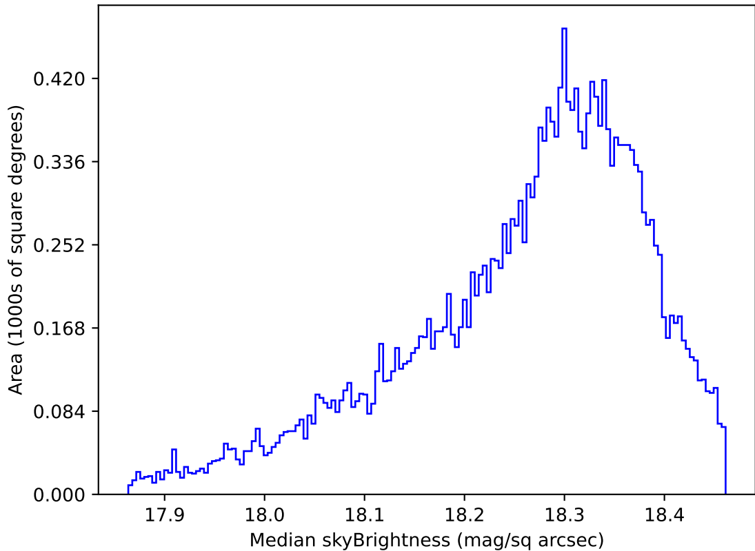
early_u_fpextra3.0_v3.4_10yrs Yr 1 y band: Median skyBrightness
