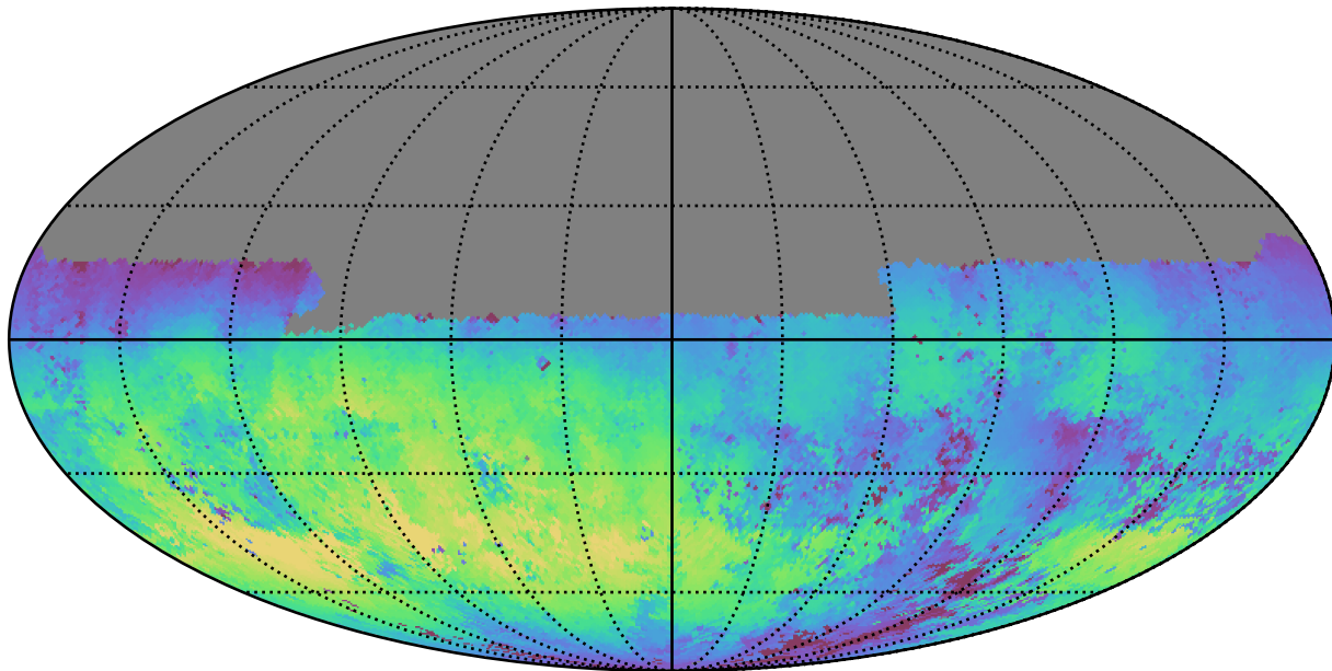
early_u_fpextra3.0_v3.4_10yrs Yr 1 u band: Median skyBrightness
