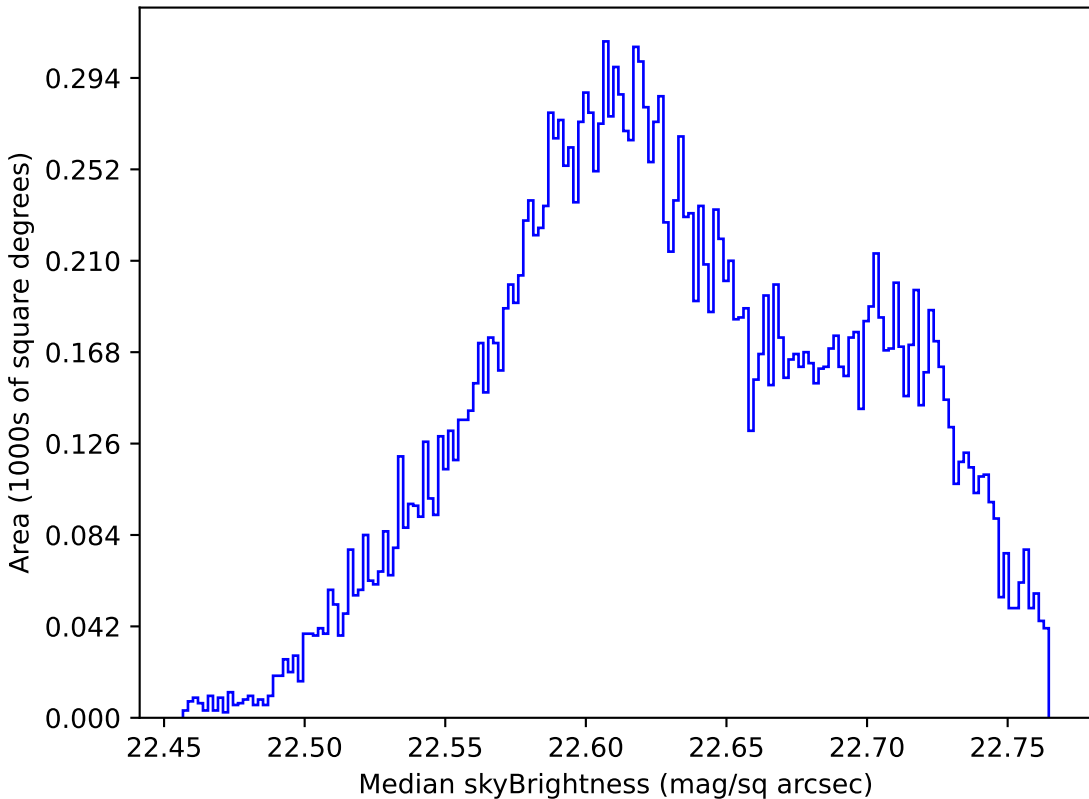
early_u_fpxextra3.0_v3.4_10yrs Yr 1 u band: Median skyBrightness
