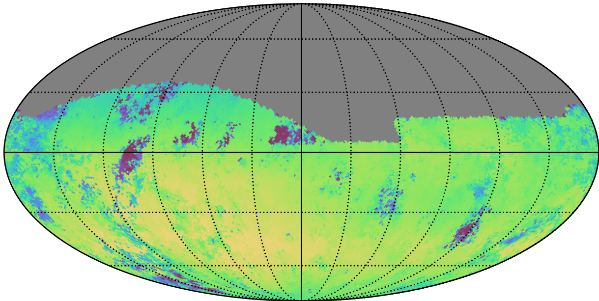
early_u_fpextra3.0_v3.4_10yrs Yr 1 r band: Median skyBrightness
