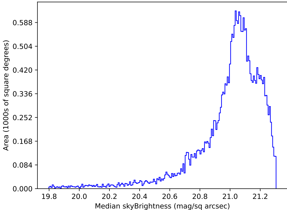
early_u_fpextra3.0_v3.4_10yrs Yr 1 r band: Median skyBrightness
