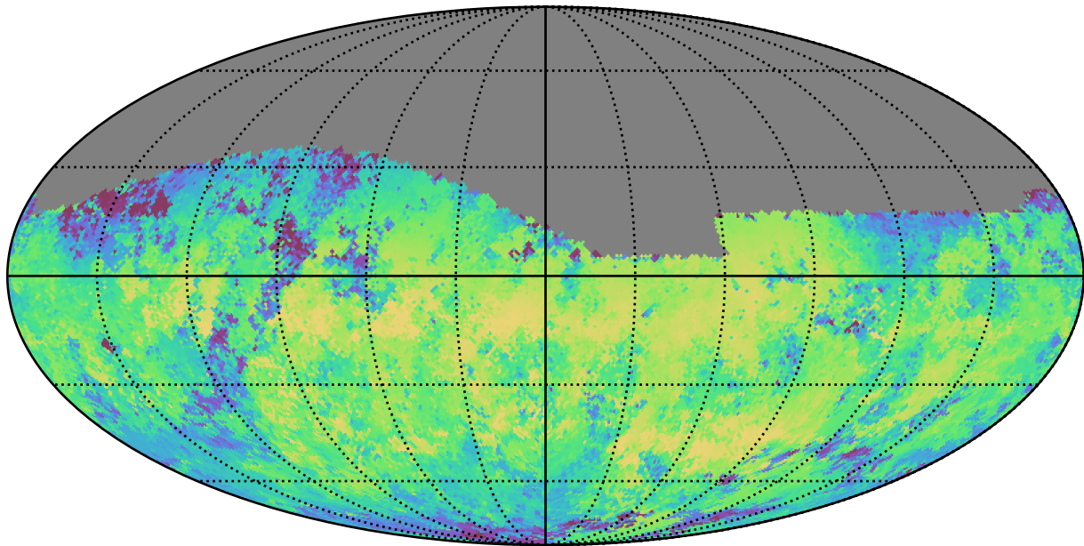
early_u_fpextra3.0_v3.4_10yrs Yr 1 i band: Median skyBrightness
