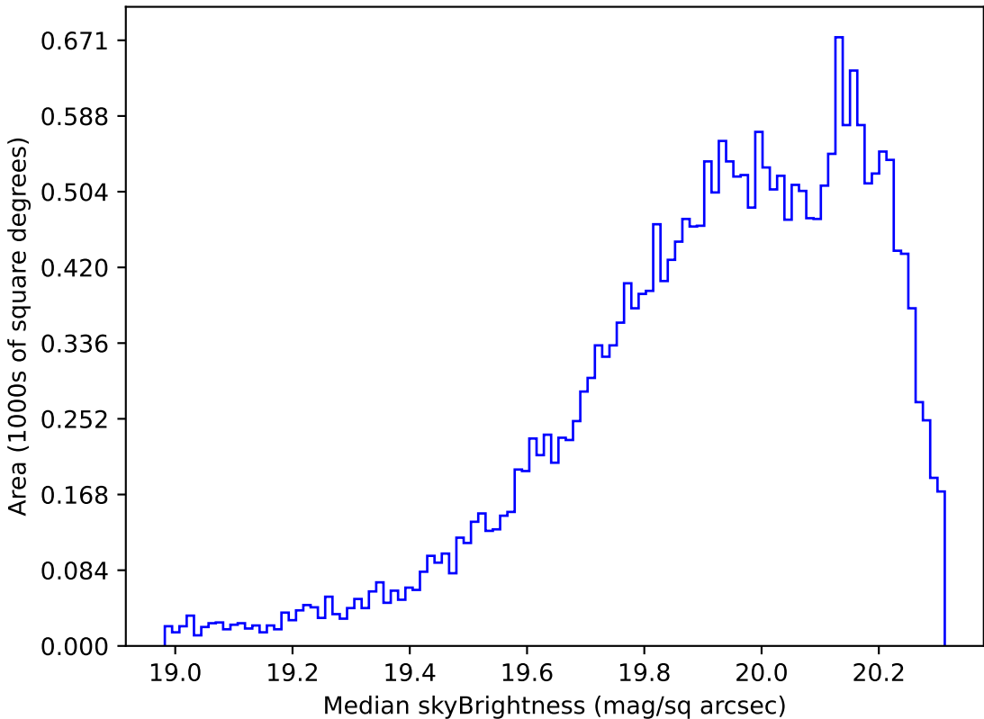
early_u_fpextra3.0_v3.4_10yrs Yr 1 i band: Median skyBrightness
