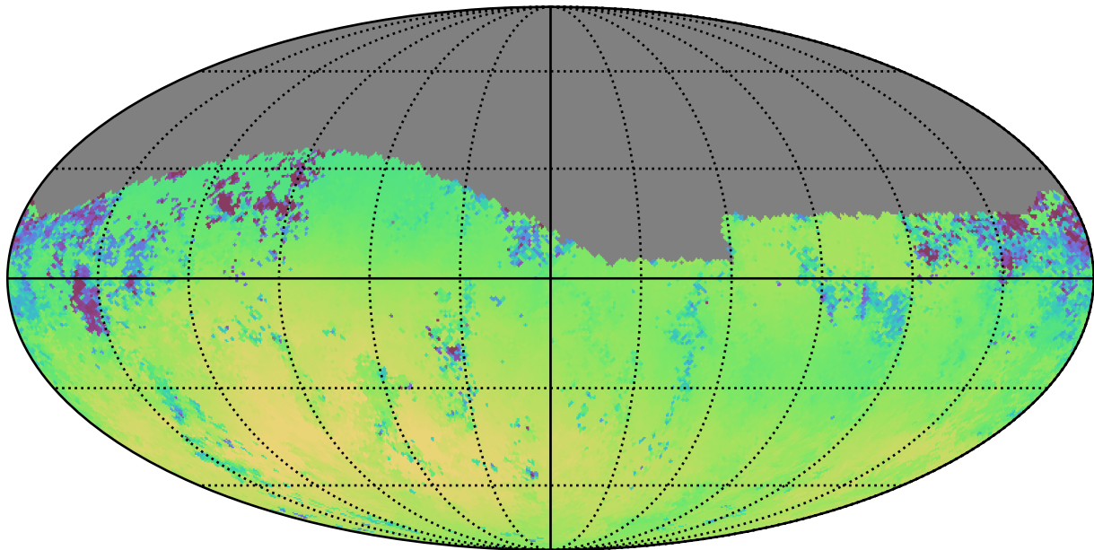
early_u_fpextra3.0_v3.4_10yrs Yr 1 g band: Median skyBrightness
