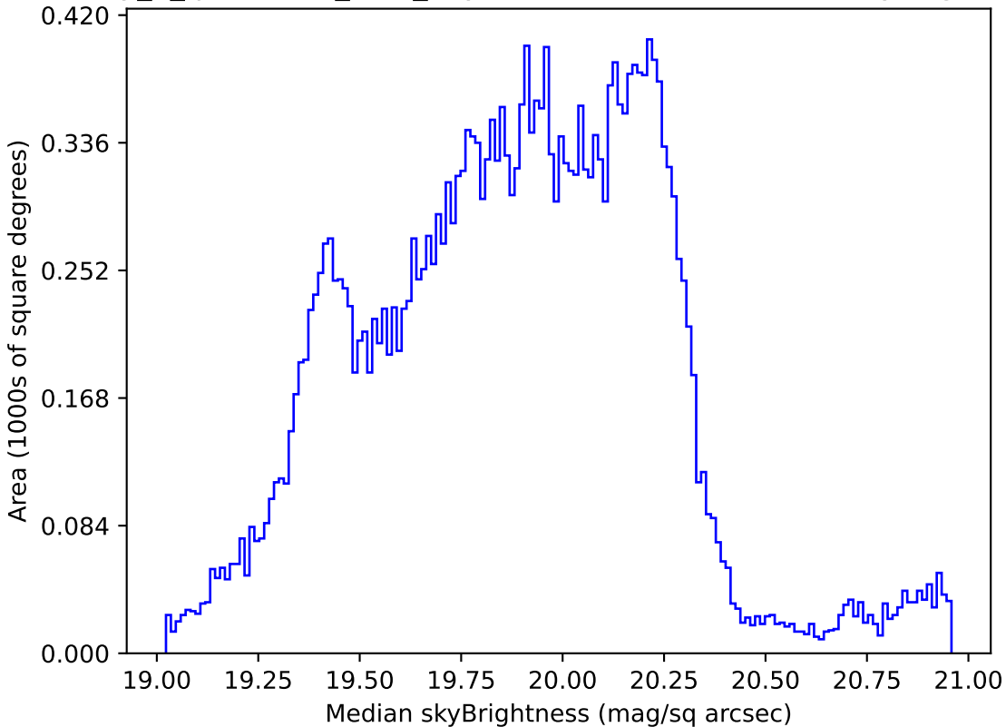
early_u_fpextra3.0_v3.4_10yrs Yr 1 all bands: Median skyBrightness
