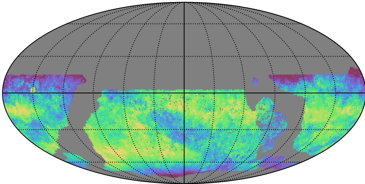
early_u_fpextra3.0_v3.4_10yrs WFD z band: Median skyBrightness
