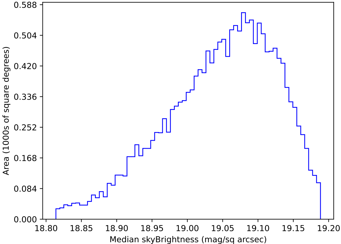
early_u_fpextra3.0_v3.4_10yrs WFD z band: Median skyBrightness
