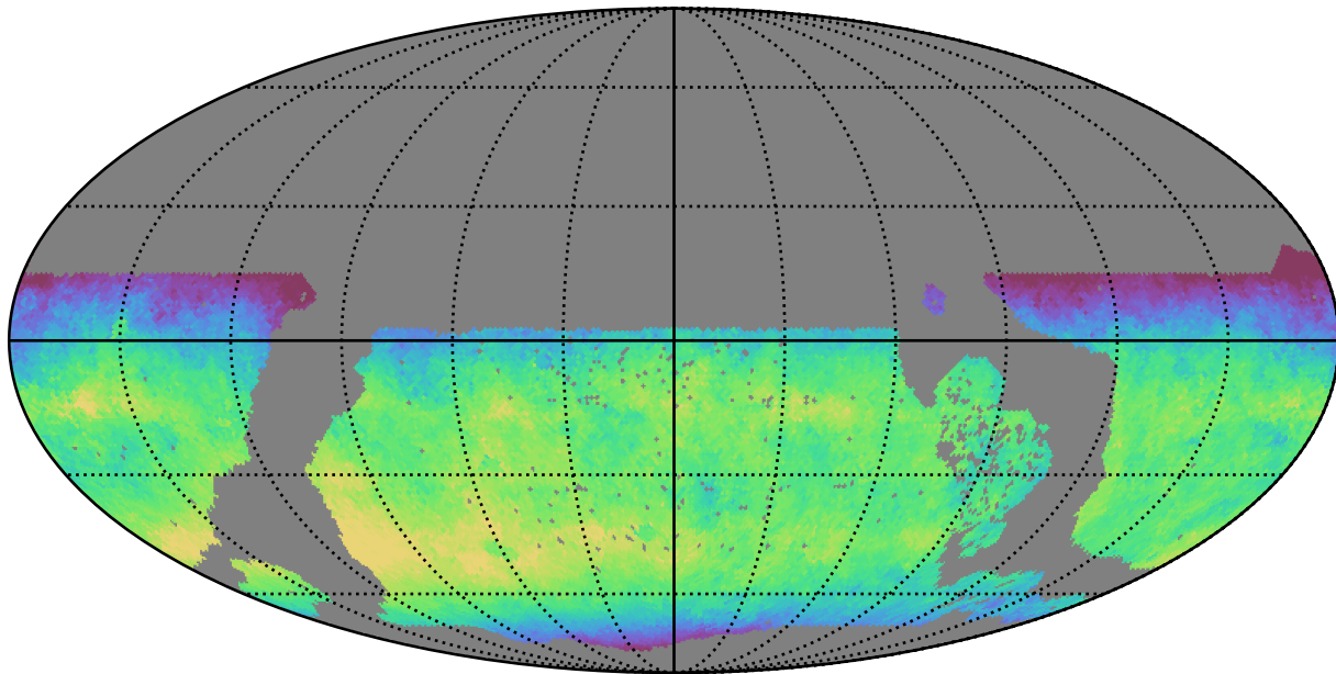
early_u_fpextra3.0_v3.4_10yrs WFD y band: Median skyBrightness
