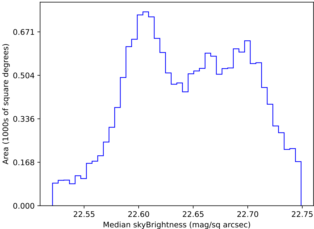
early_u_fpextra3.0_v3.4_10yrs WFD u band: Median skyBrightness
