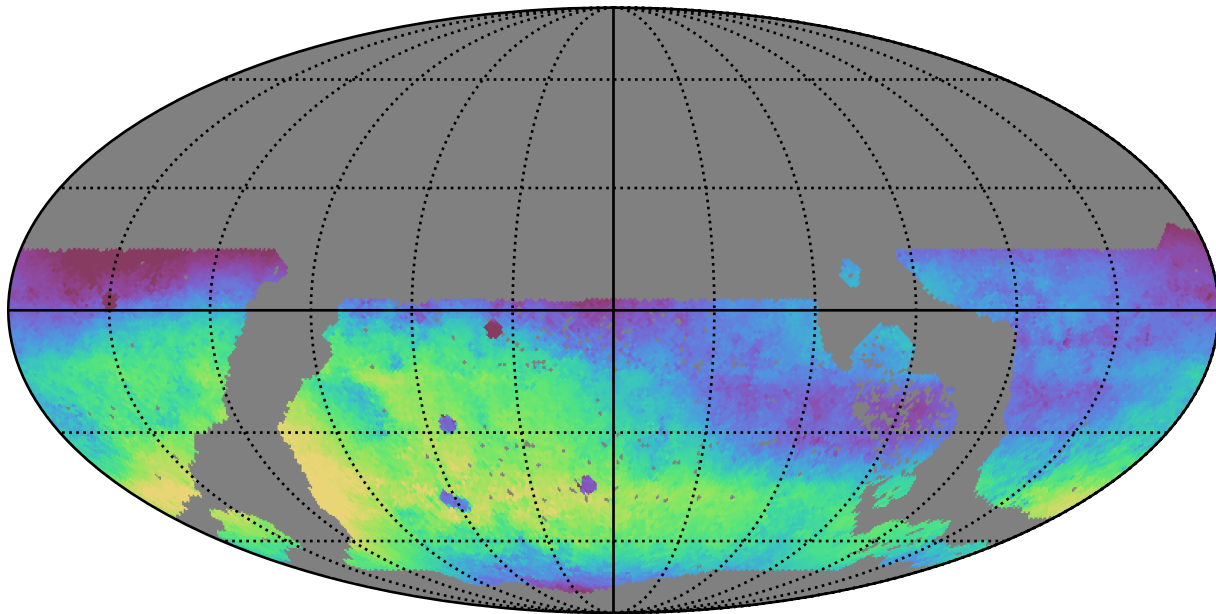
early_u_fpextra3.0_v3.4_10yrs WFD r band: Median skyBrightness
