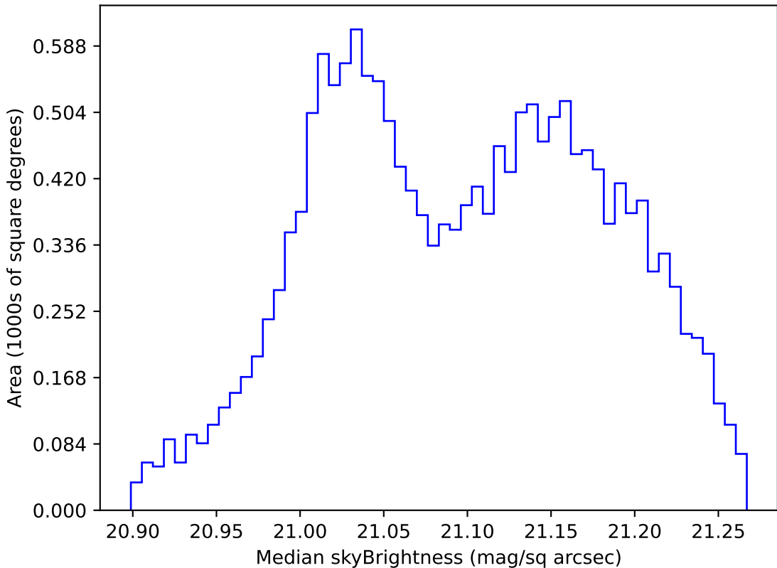
early_u_fpextra3.0_v3.4_10yrs WFD r band: Median skyBrightness
