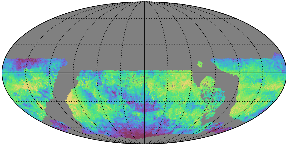
early_u_fpextra3.0_v3.4_10yrs WFD i band: Median skyBrightness
