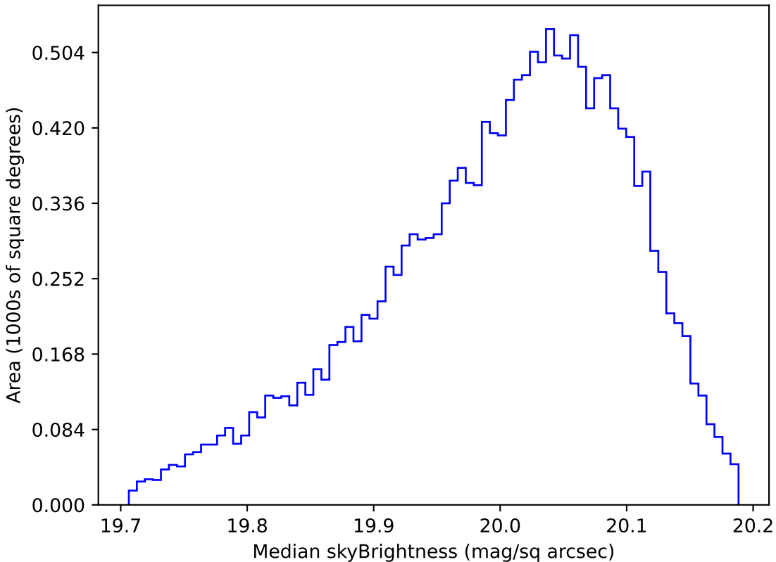
early_u_fpextra3.0_v3.4_10yrs WFD i band: Median skyBrightness
