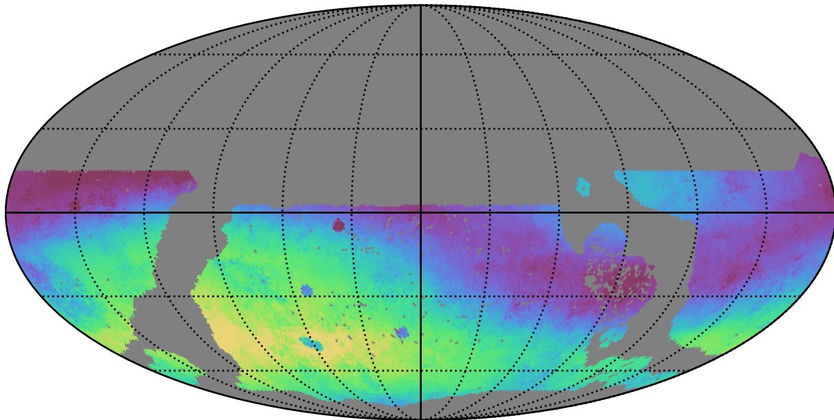
early_u_fpextra3.0_v3.4_10yrs WFD g band: Median skyBrightness
