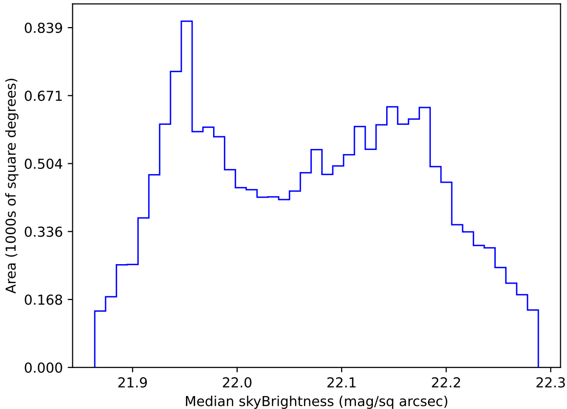
early_u_fpextra3.0_v3.4_10yrs WFD g band: Median skyBrightness
