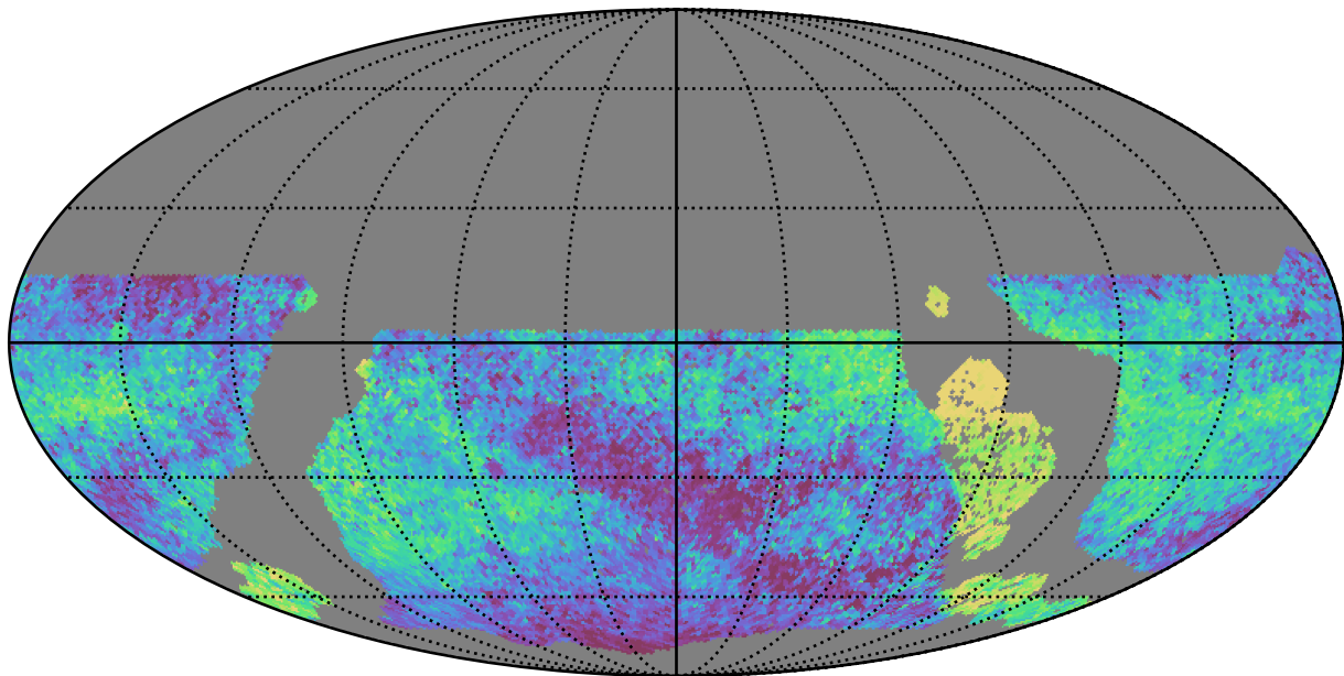
early_u_fpextra3.0_v3.4_10yrs WFD all bands: Median skyBrightness
