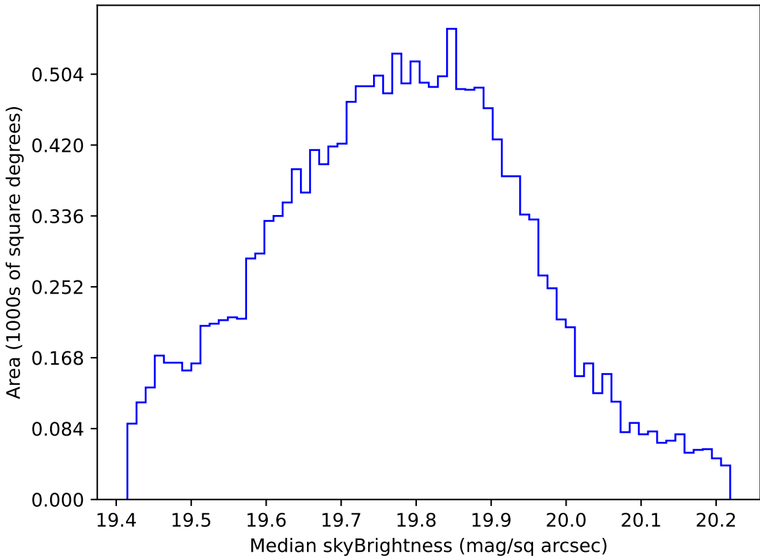
early_u_fpextra3.0_v3.4_10yrs WFD all bands: Median skyBrightness
