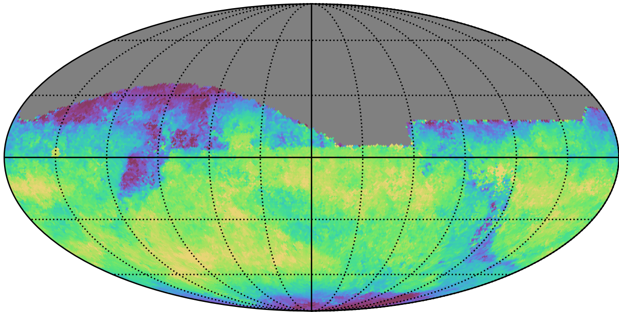
early_u_fpextra3.0_v3.4_10yrs All sky z band: Median skyBrightness
