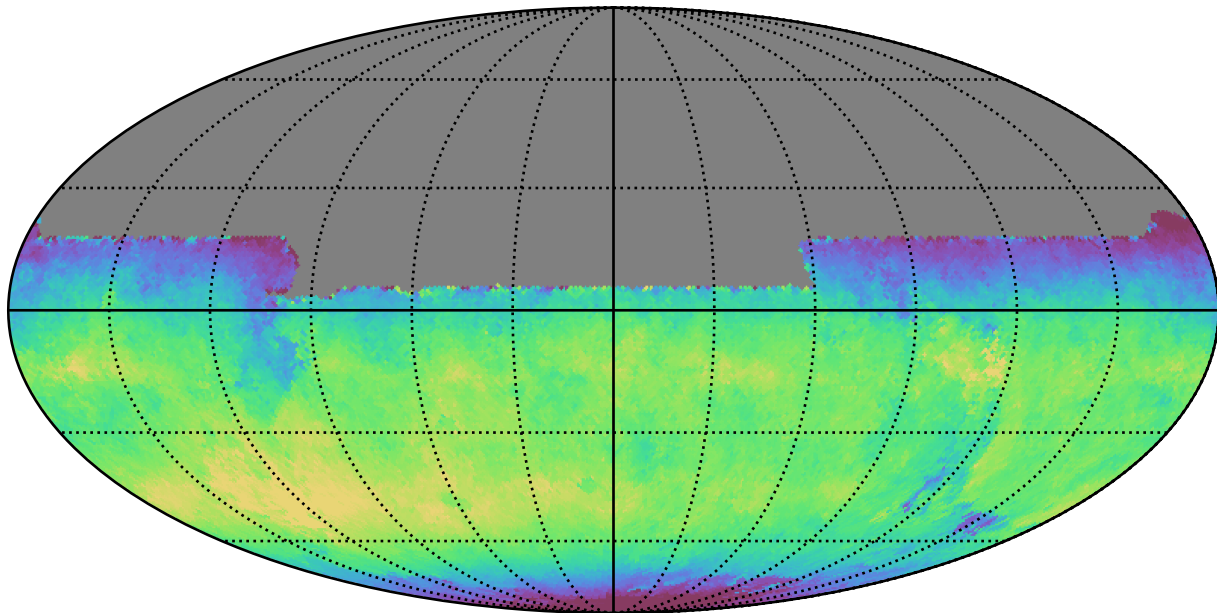
early_u_fpextra3.0_v3.4_10yrs All sky y band: Median skyBrightness
