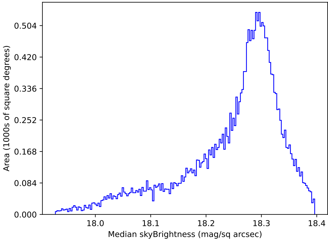
early_u_fpextra3.0_v3.4_10yrs All sky y band: Median skyBrightness
