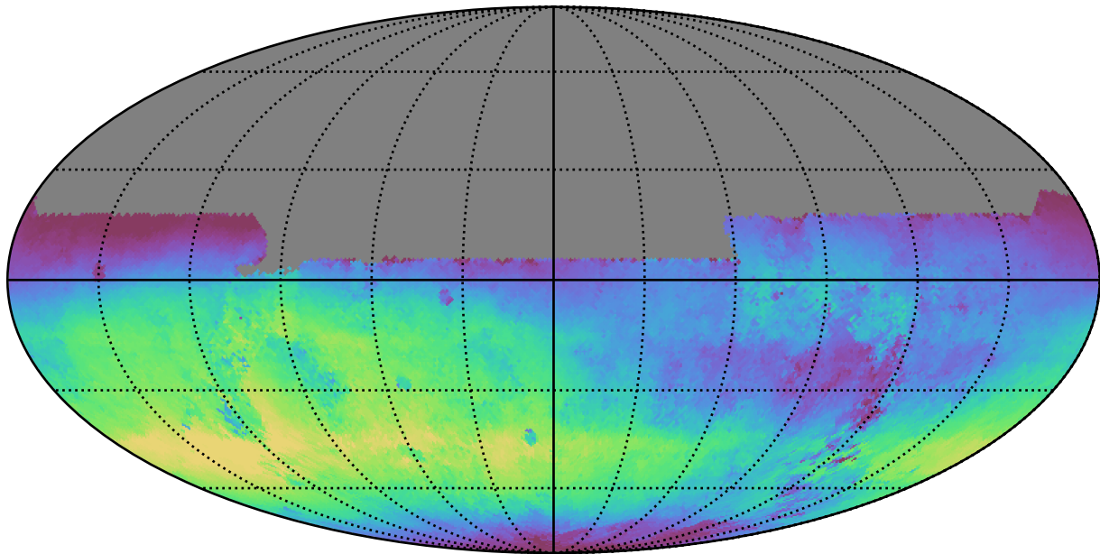
early_u_fpextra3.0_v3.4_10yrs All sky u band: Median skyBrightness
