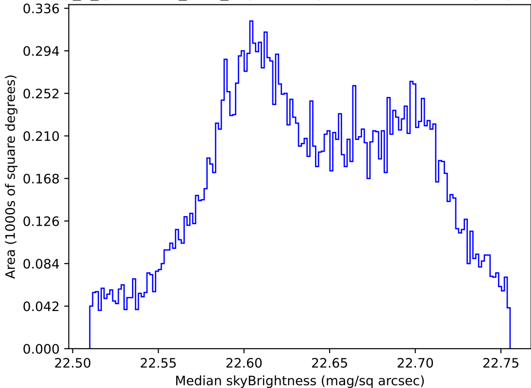
early_u_fpextra3.0_v3.4_10yrs All sky u band: Median skyBrightness
