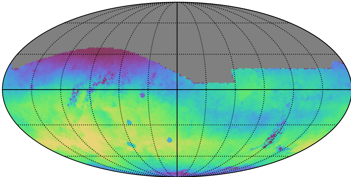
early_u_fpextra3.0_v3.4_10yrs All sky r band: Median skyBrightness
